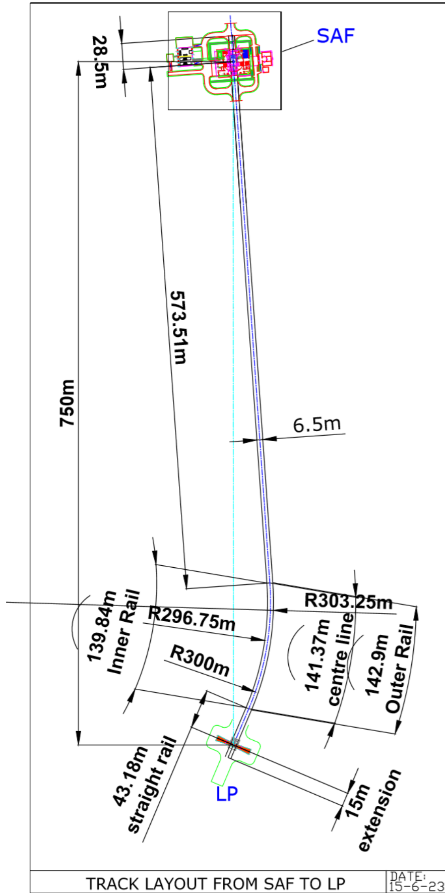
Fig 1: Details of Rail track system layout
